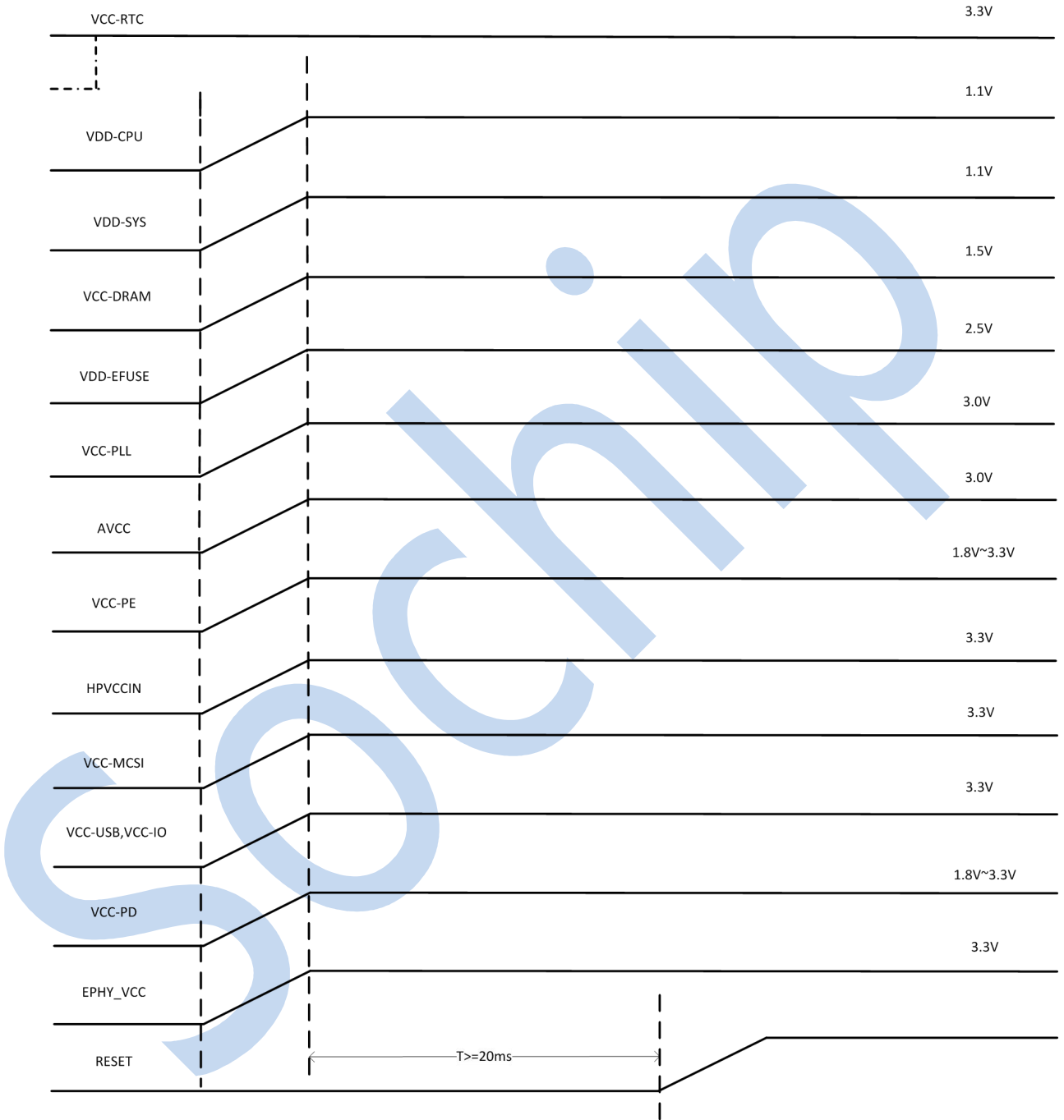
Figure 9-1. Power On Sequence
