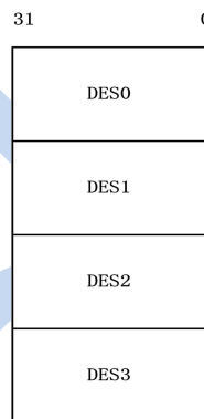
Figure 5-4. Internal Formats of A Descriptor
