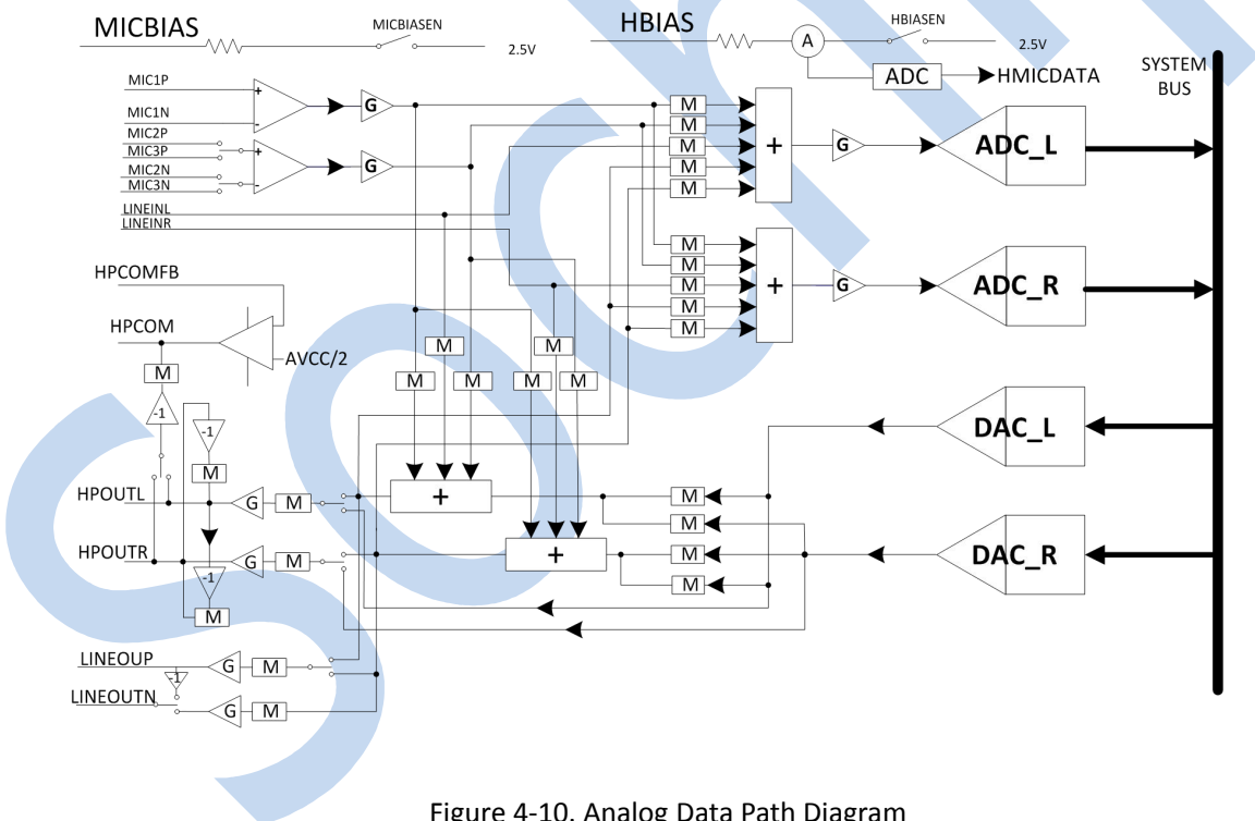
Figure 4-10. Analog Data Path Diagram
