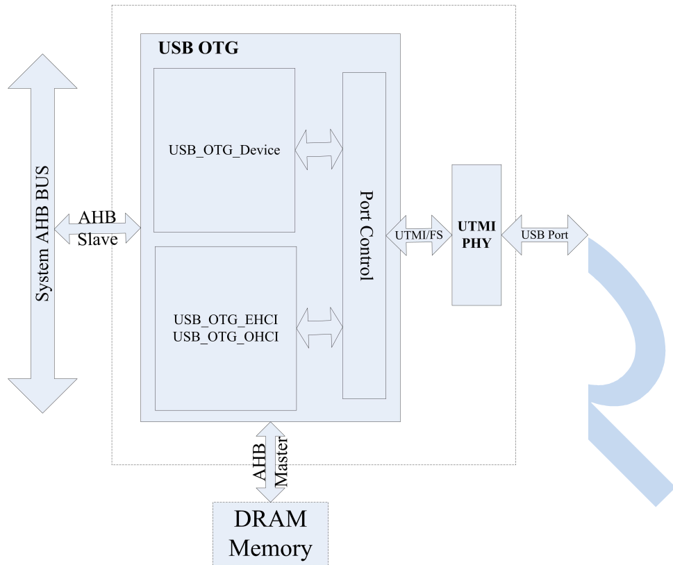
Figure 8-6. USB OTG Controller Block Diagram
